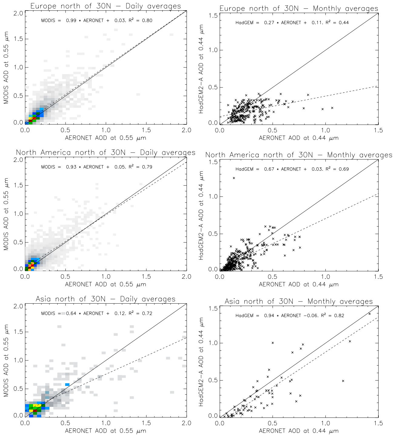
Figure 7. Left: daily-averaged total aerosol optical depth at 0.55 μm from MODIS MOD08_D3 collection 5 against that from AERONET version 2 level 2.0 for 2002. Coloured boxes indicate the percentage of total points in aerosol optical depth bins of 0.05 by 0.05. Right: monthly total aerosol optical depth at 0.44 μm from HadGEM2-A against that from AERONET. AERONET sites are listed in Table 3. Values from MODIS and HadGEM2-A are those for the gridbox that contains the AERONET site. The 1-to-1 line is the solid line, and the best linear fit is indicated by the dashed line.
